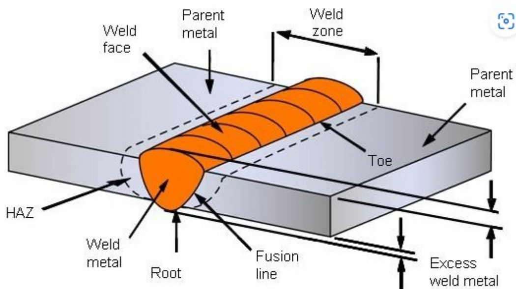
Butt weld diagram
