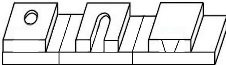
Plug Welding
